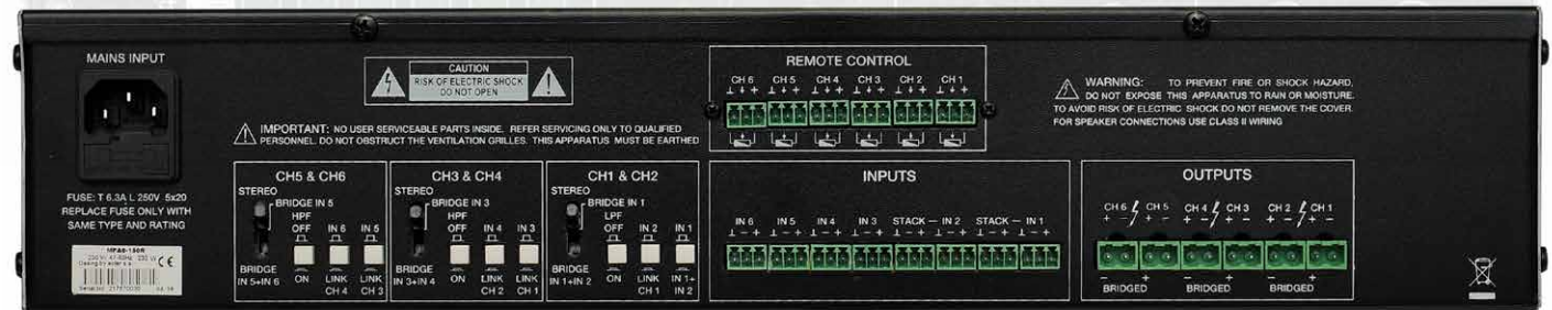
4-150R and 6-150R back panel connectors and switches style
